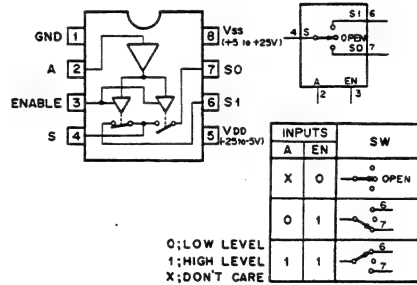
SN72607P (TI) TL607CP (TI) TL607CPS (TI) FLAT PACKAGE P-MOS ANALOG SWITCH — TOP VIEW —
